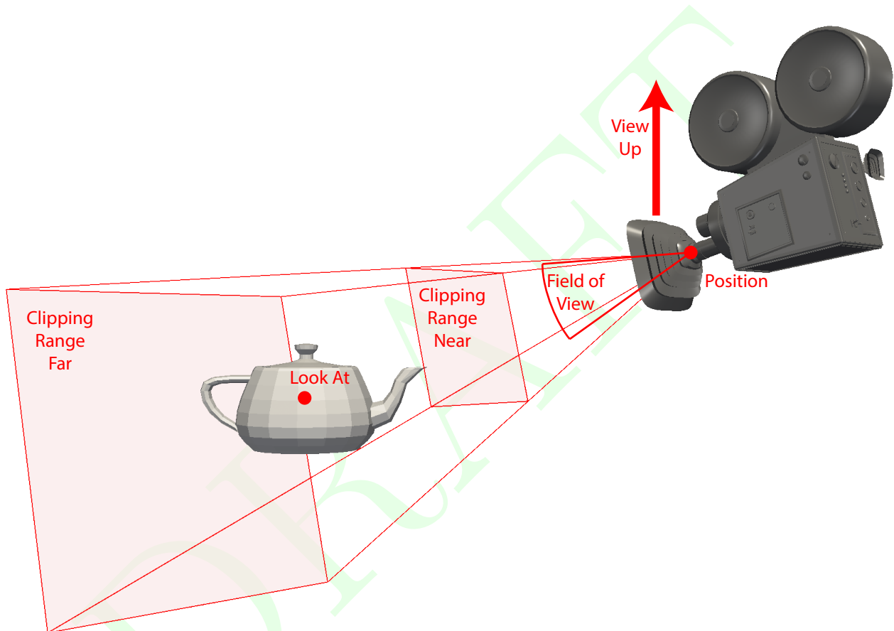
Figure 4.3: The position and orientation parameters for a Camera .
