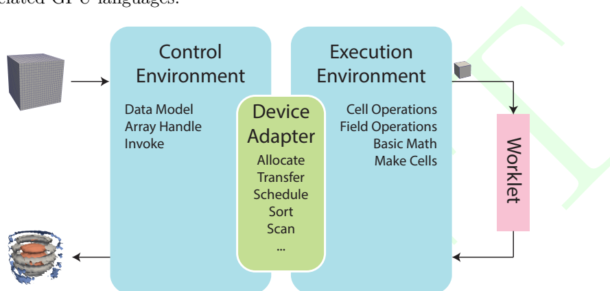
Figure 5.1: Diagram of the VTK-m framework.
