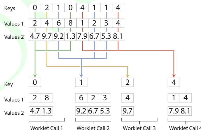
Figure 14.2: The collection of values for a reduce by key worklet.
