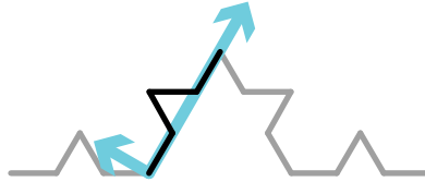
Figure 24.4: Applying the line fractal transform for the Koch Snowflake.
