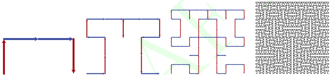
Figure 24.9: The first, second, third, and sixth iterations, respectively, of the Hilbert curve fractal.
