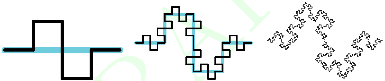
Figure 24.5: The quadratic type 2 curve fractal. The left image gives the first iteration. The middle image gives the second iteration. The right image gives the result after a few iterations.
