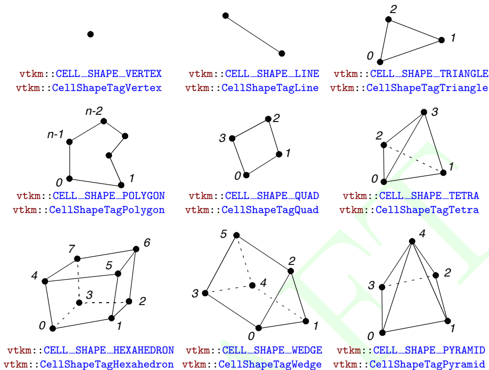
Figure 16.1: Basic Cell Shapes
