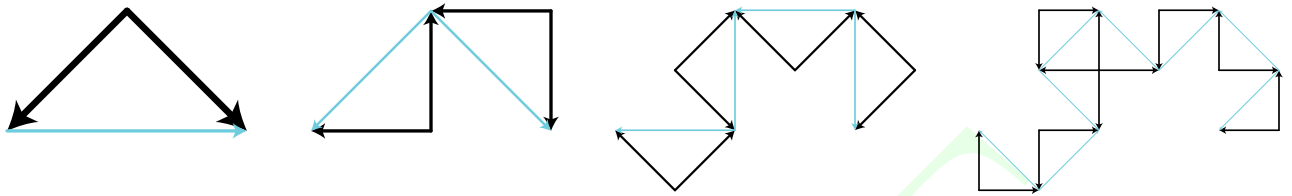
Figure 24.7: The first four iterations of the dragon fractal. The cyan lines give the previous iteration for reference.
