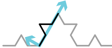
Figure 25.4: Applying the line fractal transform for the Koch Snowflake.
