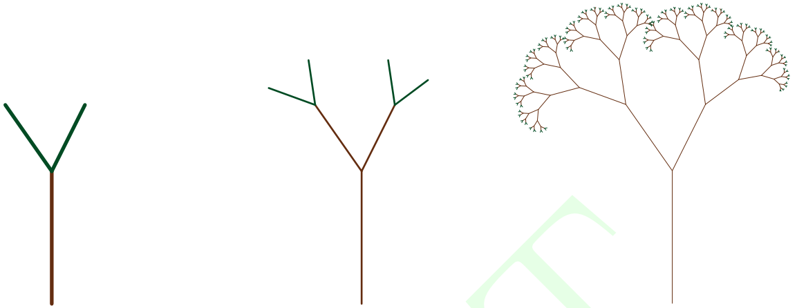
Figure 25.6: The tree fractal replaces each line with the “Y” shape shown at left. An iteration grows branches at the end (middle). After several iterations the tree branches out to the bushy shape at right.
