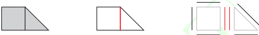
Figure 18.1: Duplicate lines from extracted edges. Consider the small mesh at the left comprising a square and a triangle. If we count the edges in this mesh, we would expect to get 6. However, our naïve implementation in Section 18.1 generates 7 because the shared edge (highlighted in red in the wireframe in the middle) is duplicated. As seen in the exploded view at right, one line is created for the square and one for the triangle.
