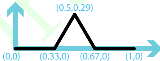
Figure 25.3: Parametric coordinates for the Koch Snowflake shape.
