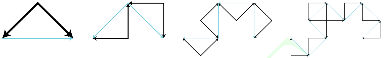
Figure 25.7: The first four iterations of the dragon fractal. The cyan lines give the previous iteration for reference.
