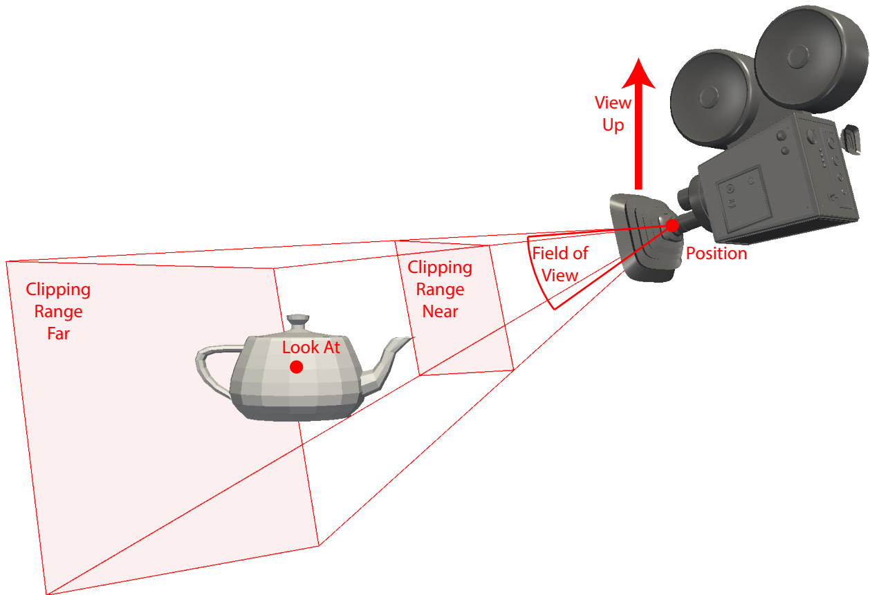
Figure 5.3: The position and orientation parameters for a Camera .
