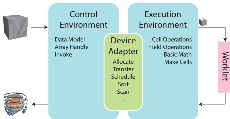
Figure 6.1: Diagram of the VTK-m framework.
