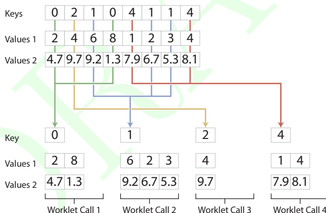
Figure 13.2: The collection of values for a reduce by key worklet.
