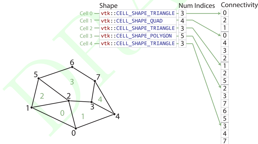
Figure 12.1: An example explicit mesh.
