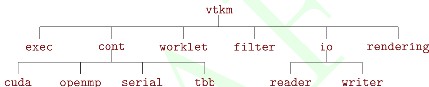
Figure 6.2: VTK-m package hierarchy.
