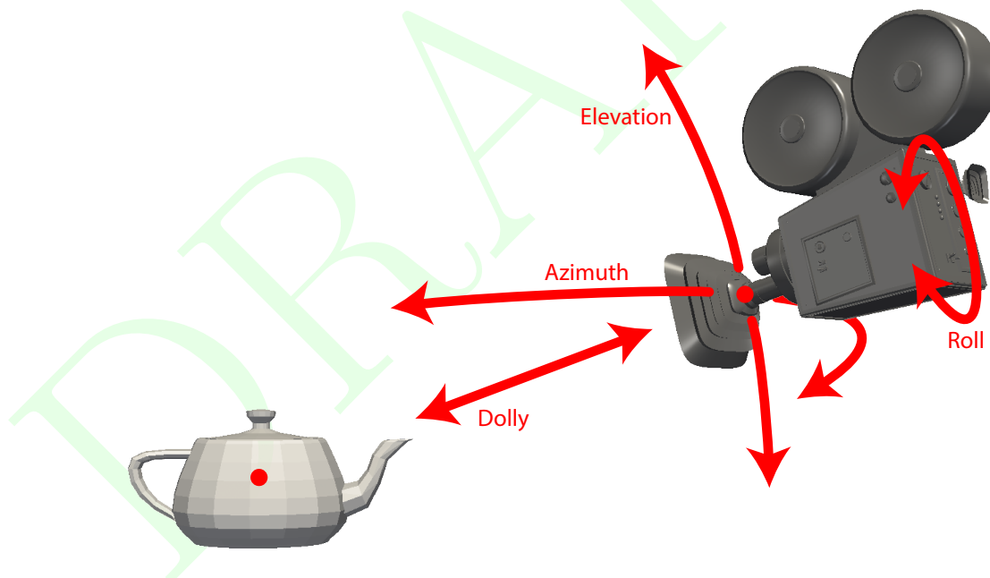
Figure 5.5: Camera movement functions relative to position and orientation.
