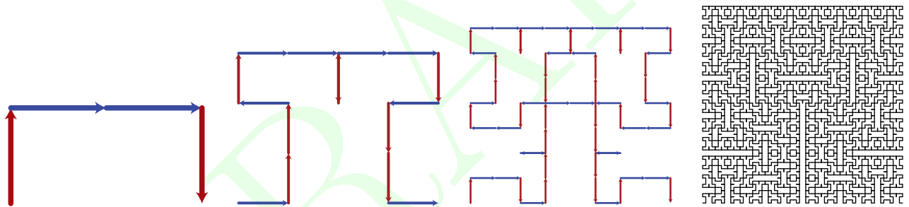
Figure 31.9: The first, second, third, and sixth iterations, respectively, of the Hilbert curve fractal.
