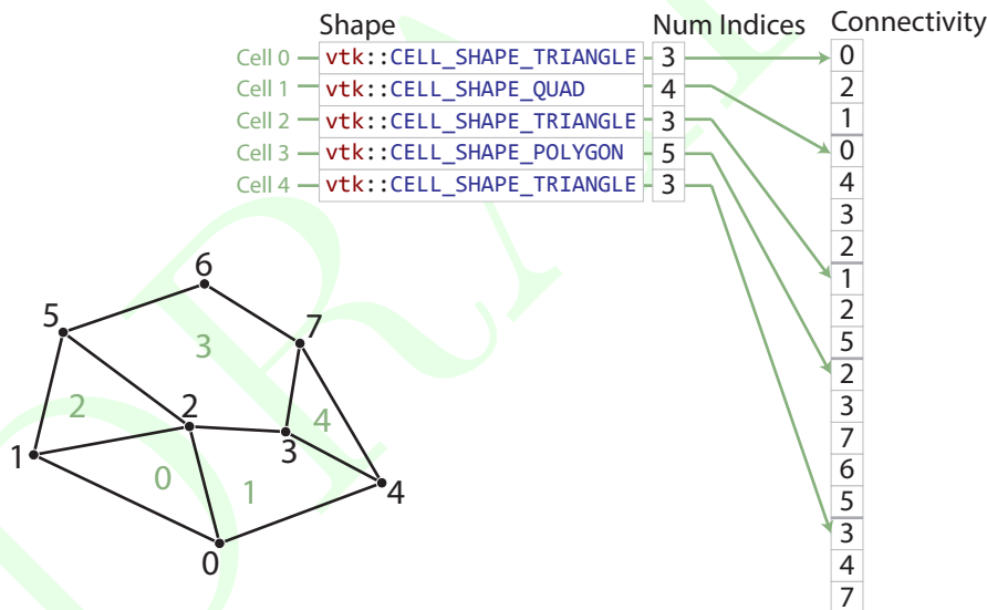
Figure 14.1: An example explicit mesh.
