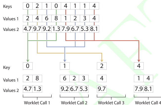
Figure 18.2: The collection of values for a reduce by key worklet.
