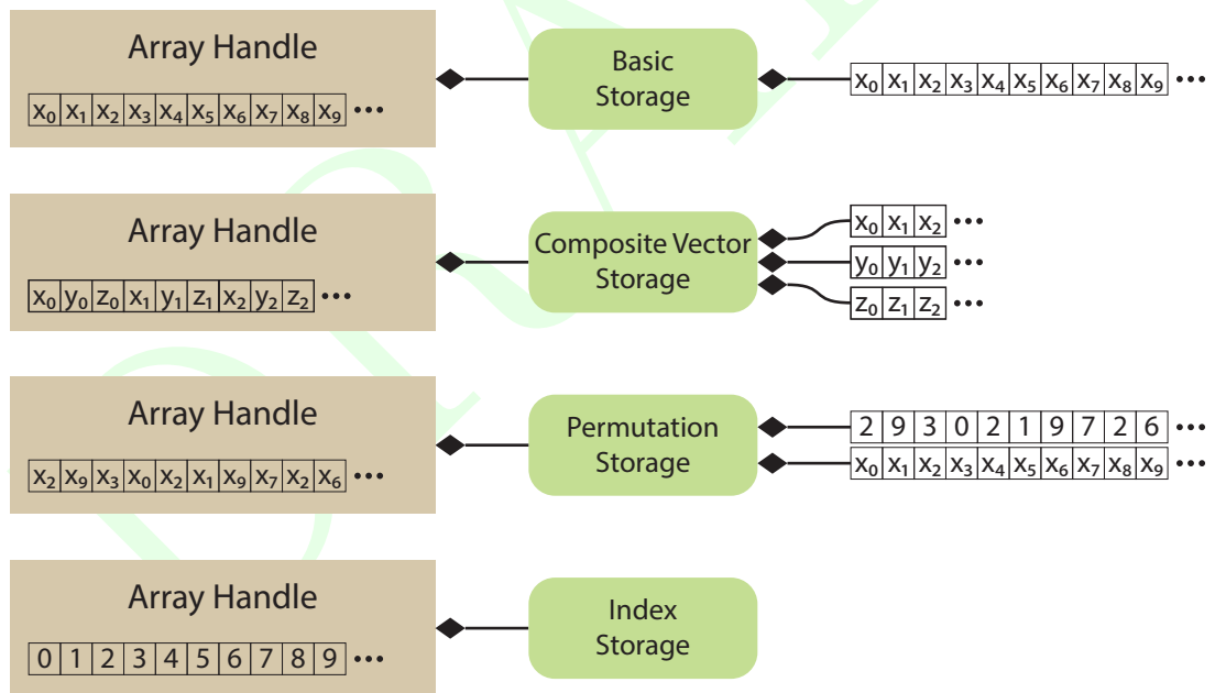
Figure 26.1: Array handles, storage objects, and the underlying data source.
