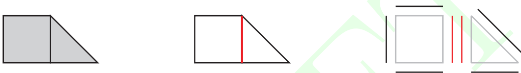
Figure 22.1: Duplicate lines from extracted edges. Consider the small mesh at the left comprising a square and a triangle. If we count the edges in this mesh, we would expect to get 6. However, our naïve implementation in Section 22.1 generates 7 because the shared edge (highlighted in red in the wireframe in the middle) is duplicated. As seen in the exploded view at right, one line is created for the square and one for the triangle.
