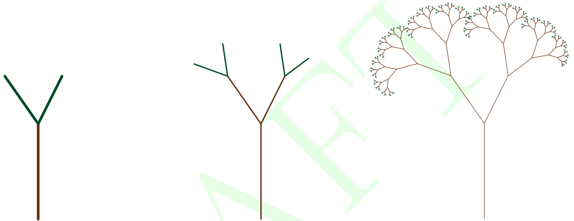
Figure 31.6: The tree fractal replaces each line with the “Y” shape shown at left. An iteration grows branches at the end (middle). After several iterations the tree branches out to the bushy shape at right.
