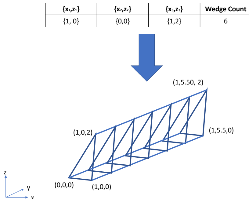
Figure 14.5: An example of an extruded wedge from XZ-plane coordinates. Six wedges are extracted from three XZ-plane points.
