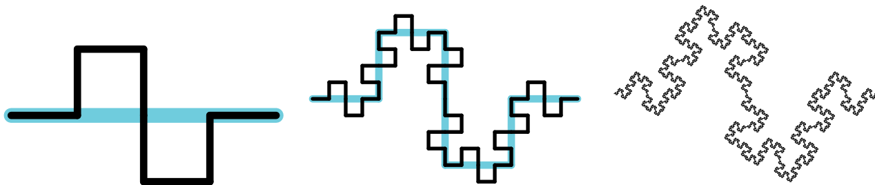
Figure 31.5: The quadratic type 2 curve fractal. The left image gives the first iteration. The middle image gives the second iteration. The right image gives the result after a few iterations.
