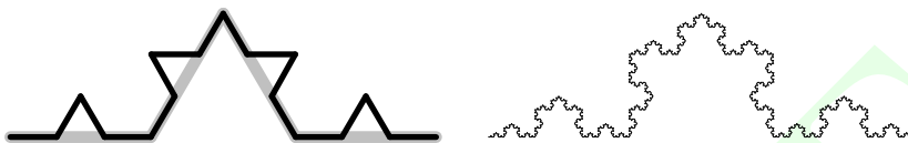
Figure 31.2: The Koch Snowflake after the second iteration (left image) and after several more iterations (right image).
