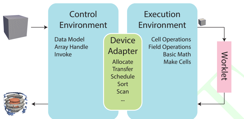
Figure 17.1: Diagram of the VTK-m framework.
