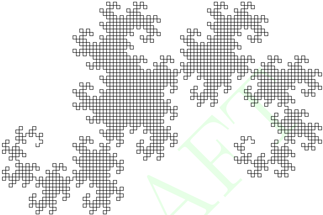
Figure 31.8: The dragon fractal after 12 iterations.
