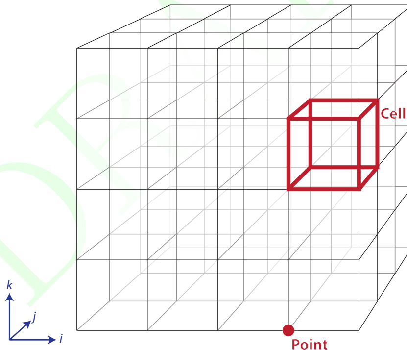
Figure 14.3: The arrangement of points and cells in a 3D structured grid.
